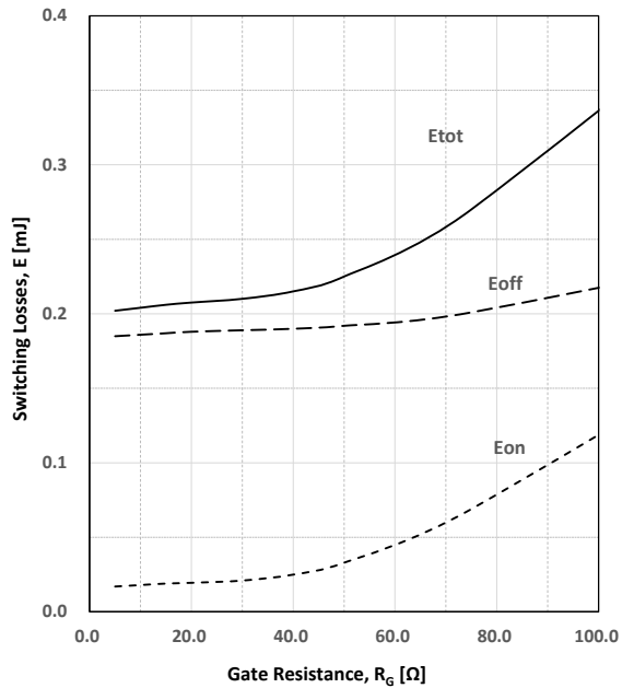
Figure.10 Switching Loss as Gate Resistance ( V_{CE}=400V, I_C=10A, V_{GE}=15V, T_J=25^\circ C )
