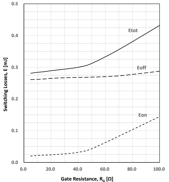
Figure.16 Switching Loss as Gate Resistance ( V_{CE}=400V , I_C=10A , V_{GE}=15V , T_J=150^\circ C )
