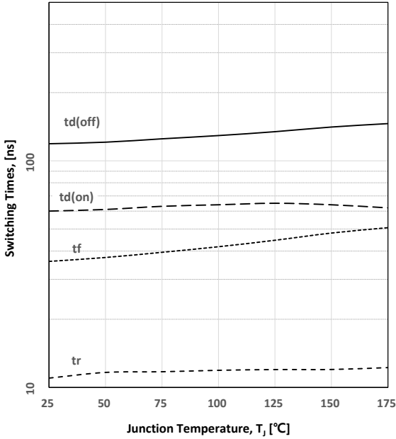
Figure.21 Switching Times as Junction Temp. ( V_{CE}=400V, I_C=20A, V_{GE}=15V, R_g=10\Omega )
