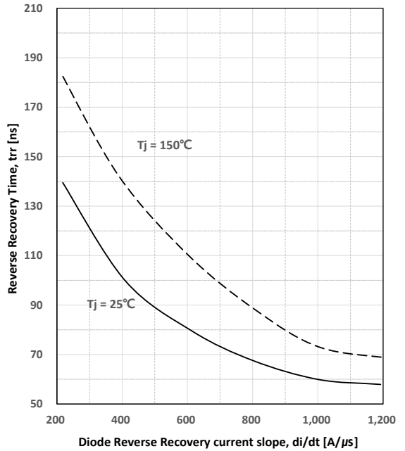
Figure.25 Reverse Recovery Time as di/dt ( V_R=400V , I_F=20A )
