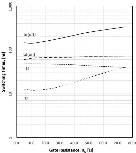
Figure.15 Switching Times as Gate Resistance ( V_{CE}=400V , I_C=20A , V_{GE}=15V , T_J=150^\circ C )
