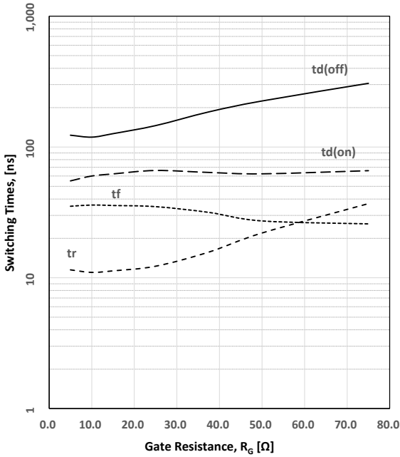
Figure.9 Switching Times as Gate Resistance ( V_{CE}=400V, I_C=20A, V_{GE}=15V, T_J=25^\circ C )
