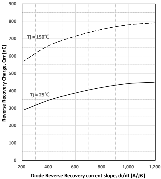
Figure.26 Reverse Recovery Charge as di/dt ( V_R=400V , I_F=20A )
