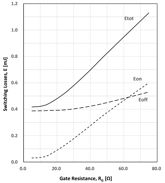
Figure.10 Switching Loss as Gate Resistance ( V_{CE}=400V, I_C=20A, V_{GE}=15V, T_J=25^\circ C )
