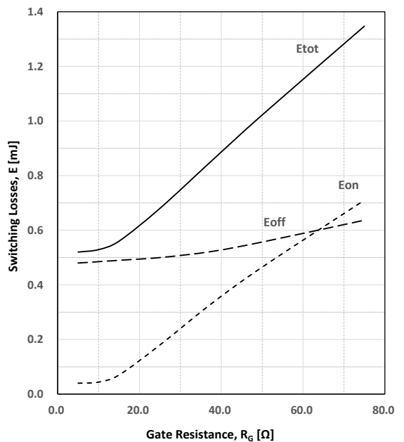
Figure.16 Switching Loss as Gate Resistance ( V_{CE}=400V , I_C=20A , V_{GE}=15V , T_J=150^\circ C )
