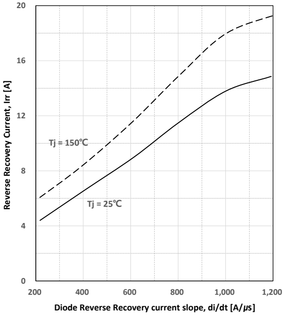
Figure.24 Reverse Recovery Current as di/dt ( V_R=400V , I_F=20A )
