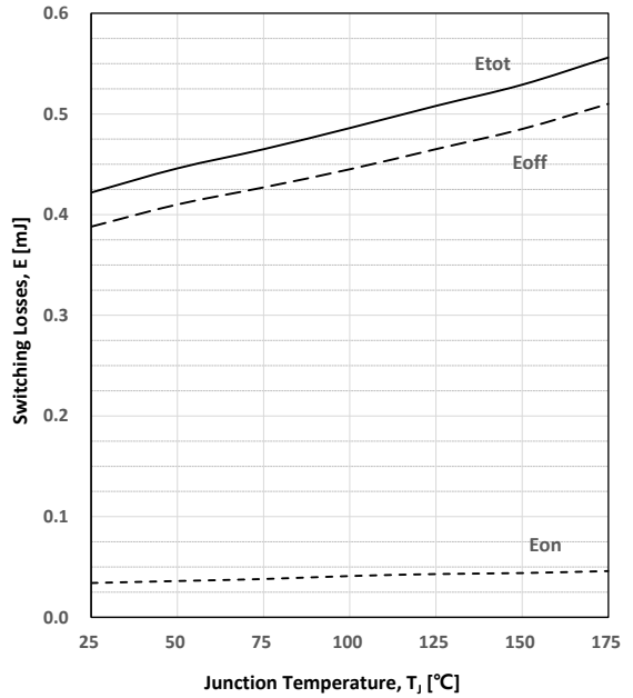
Figure.22 Switching Loss as Junction Temp. ( V_{CE}=400V, I_C=20A, V_{GE}=15V, R_g=10\Omega )
