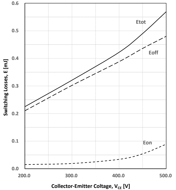
Figure.14 Switching Loss as Collector Voltage ( I_C=20A , V_{GE}=15V , R_g=10\Omega , T_J=25^\circ C )
